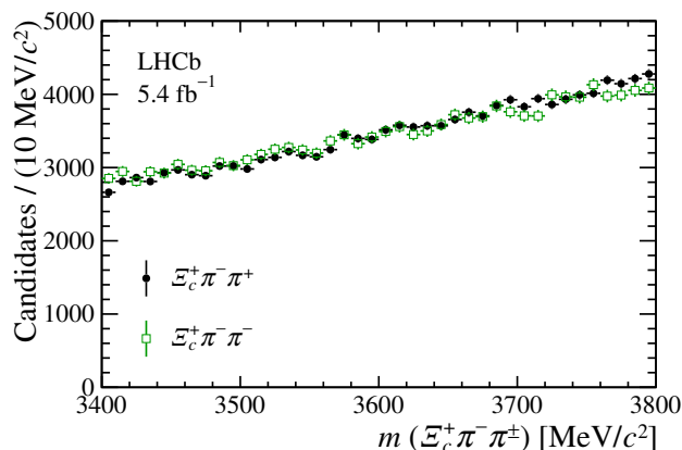
Figure 2. Invariant-mass spectrum for the \Xi_c^+\pi^-\pi^+ (black points) and the \Xi_c^+\pi^-\pi^- (green squares) final states for the default trigger set. The \Xi_c^+\pi^-\pi^- data are normalised to the \Xi_c^+\pi^-\pi^+ invariant-mass spectrum.
