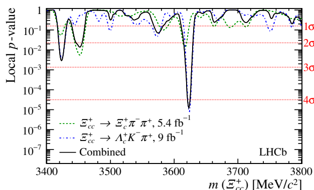
Figure 3. Local p -values as a function of the \Xi_{cc}^+ invariant mass, for \Xi_{cc}^+ baryon decays reconstructed in the \Xi_c^+\pi^-\pi^+ (green dashed curve) and \Lambda_c^+K^-\pi^+ (blue dash-dotted curve) modes, or combining the two modes (black solid curve). The horizontal dotted red lines represent the p -values corresponding to significances of 1, 2, 3 and 4 \sigma . The extended trigger set is used for the \Xi_{cc}^+\rightarrow\Xi_c^+\pi^-\pi^+ decay and Selection B from ref. [10] is used for the \Xi_{cc}^+\rightarrow\Lambda_c^+K^-\pi^+ decay. The systematic uncertainties are not taken into account.
